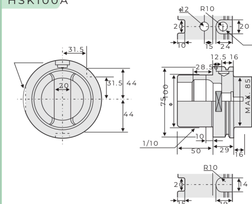
HSK100A
