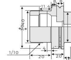
HSK40E
